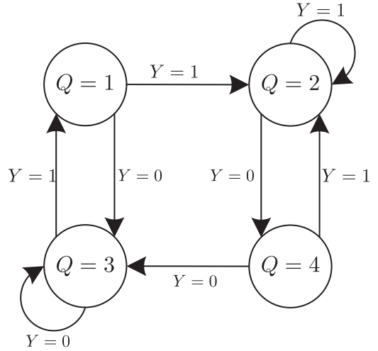
Fig. 8. Expanded Q -graph for the trapdoor channel.
