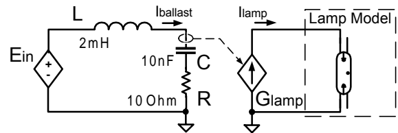
Fig. 11. Separated (tandem) scheme of ballast-lamp system (Fig. 9).
