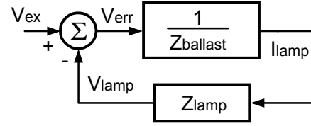
Fig. 10. Control block diagram of ballast-lamp system operating in open loop (Fig. 9)
