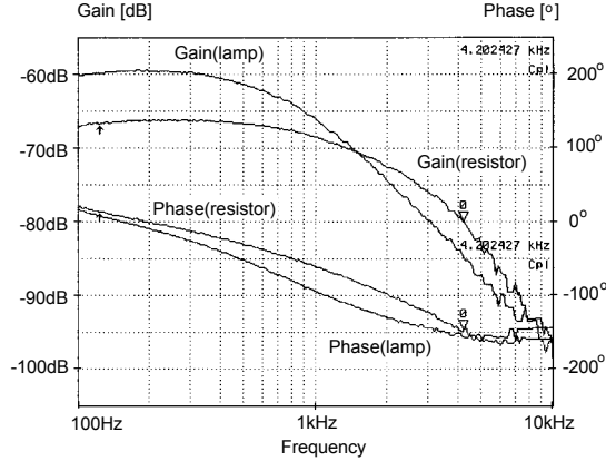
Fig. 8. Measured small signal response of the experimental ballast (Fig. 6) loaded by a resistor (150 Ohm) and a fluorescent lamp load.
