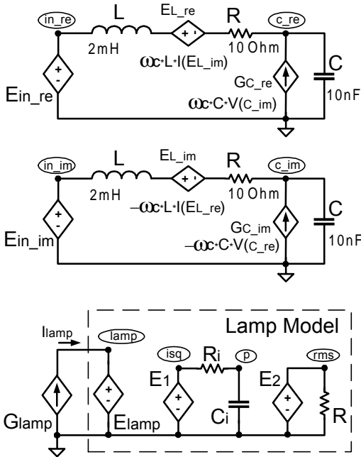
Fig. 12. Envelope simulation SPICE compatible equivalent circuits of separated ballast-lamp system operating in open loop (Fig. 11).
