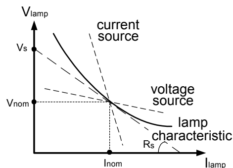
Fig. 1. The static V-I representation of high frequency ballast-lamp system operating in open loop configuration.
