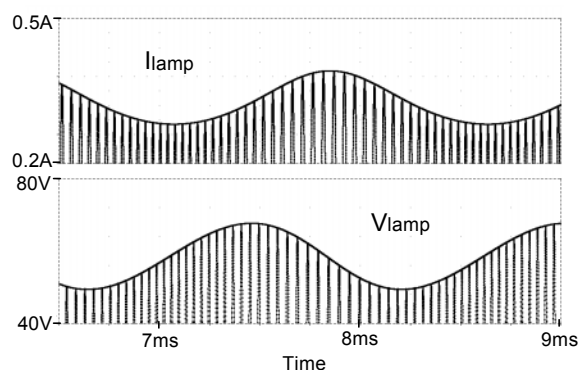
Fig. 5. Comparison of envelope and cycle-by-cycle simulation results for the circuit of Fig. 4.
