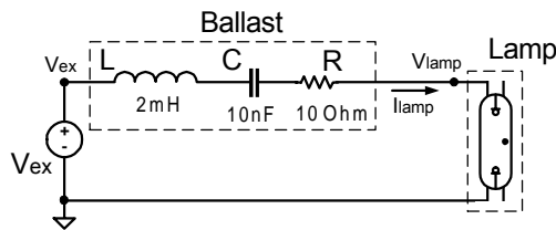
Fig. 9. Ballast-lamp system operating in open loop.
