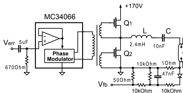
Fig. 6. Experimental ballast-lamp system.
