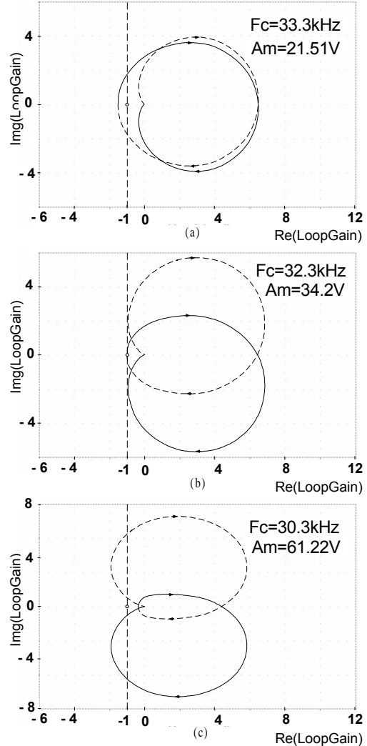
Fig. 13. Nyquist Plots of the LoopGain for different values of carrier frequency: (a) F_c = 33.3\text{kHz} . (b) F_c = 32.3\text{kHz} . (c) F_c = 30.3\text{kHz} .
