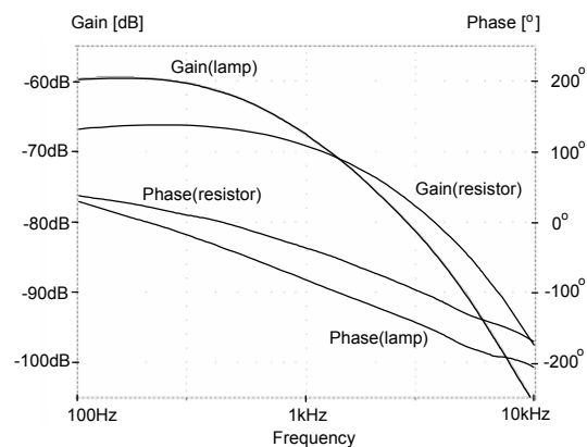
Fig. 7. Simulated small signal response of the experimental ballast (Fig. 6) loaded by a resistor (150 Ohm) and a fluorescent lamp load.
