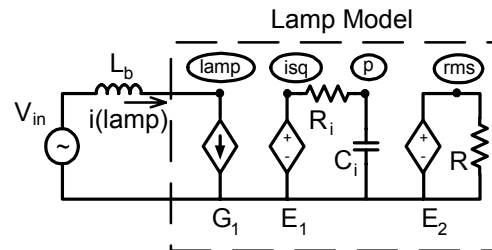
Fig. 3. SPICE compatible equivalent circuit of a fluorescent lamp. where U_1(t) and U_2(t) are the modulation signals and \omega_c is the angular frequency of the carrier.
