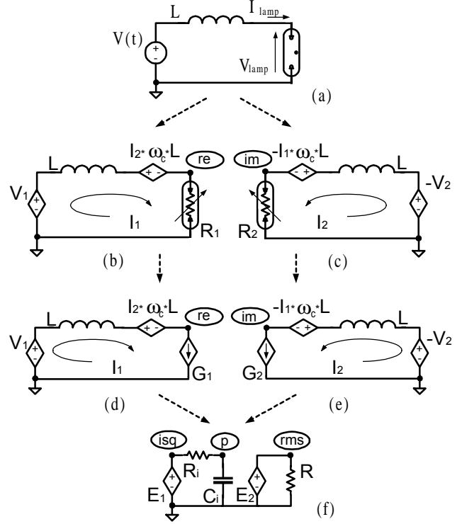
Fig. 4. SPICE compatible model used to run envelope simulation of a ballast-lamp system.
